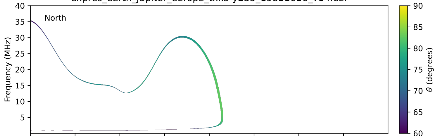
expres_earth_jupiter_europa_txka-y235_19821026_v14.cdf
