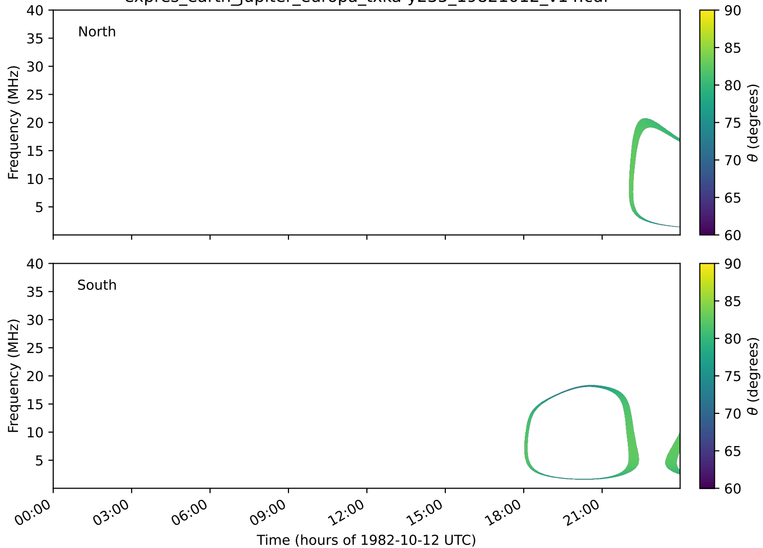
expres_earth_jupiter_europa_txka-y235_19821012_v14.cdf
