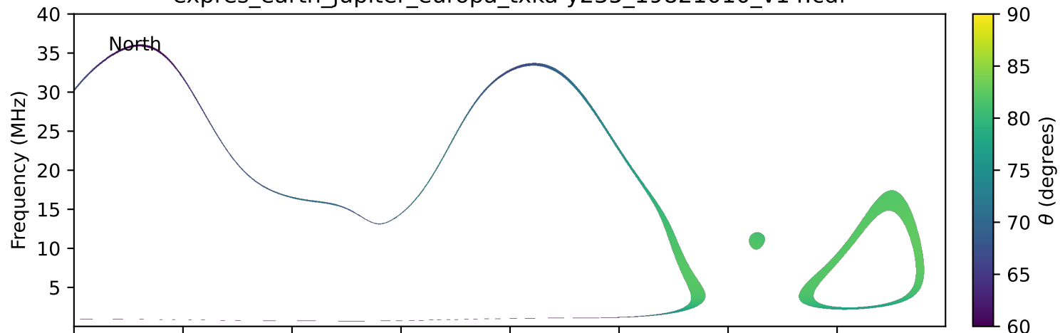
expres_earth_jupiter_europa_txka-y235_19821010_v14.cdf
