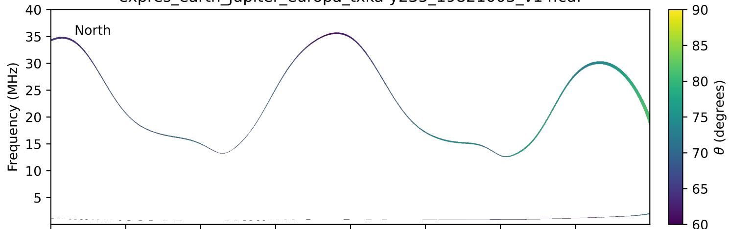
expres_earth_jupiter_europa_txka-y235_19821003_v14.cdf
