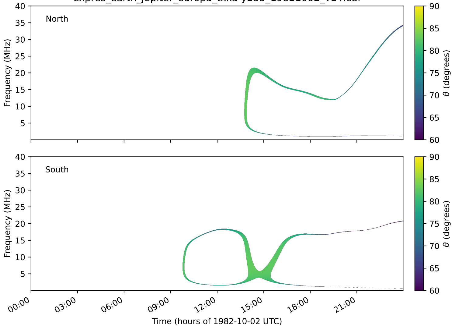
expres_earth_jupiter_europa_txka-y235_19821002_v14.cdf
