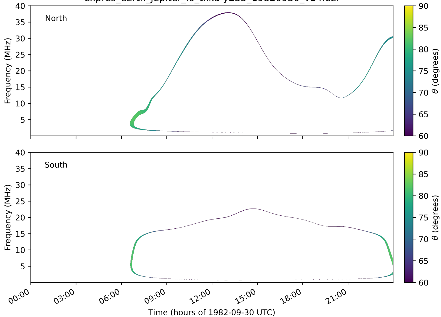
expres_earth_jupiter_io_txka-y235_19820930_v14.cdf
