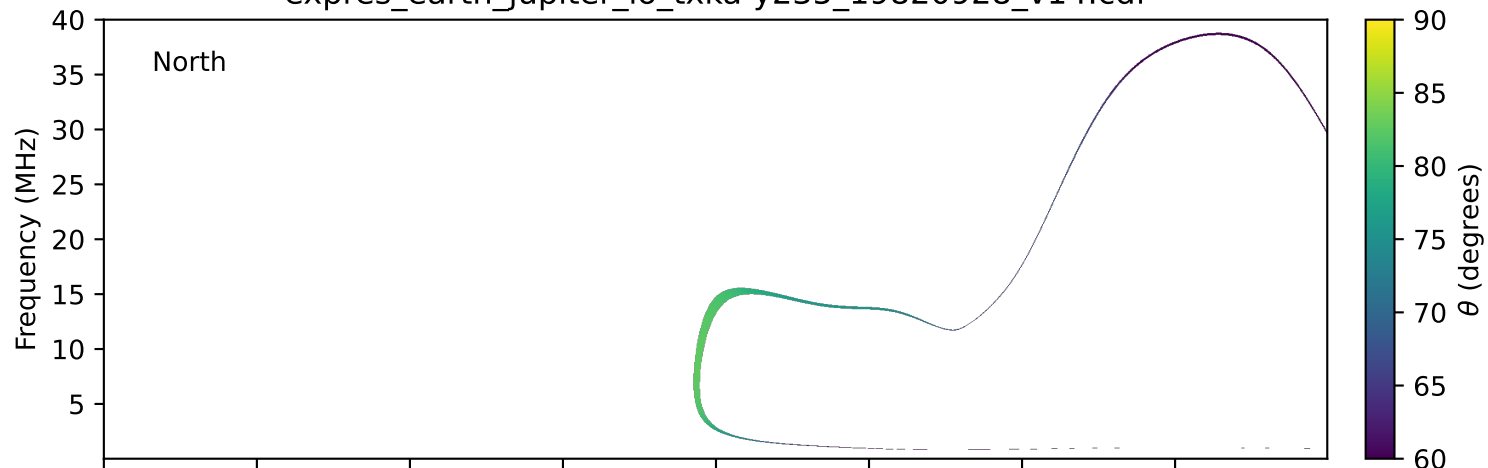
expres_earth_jupiter_io_txka-y235_19820928_v14.cdf
