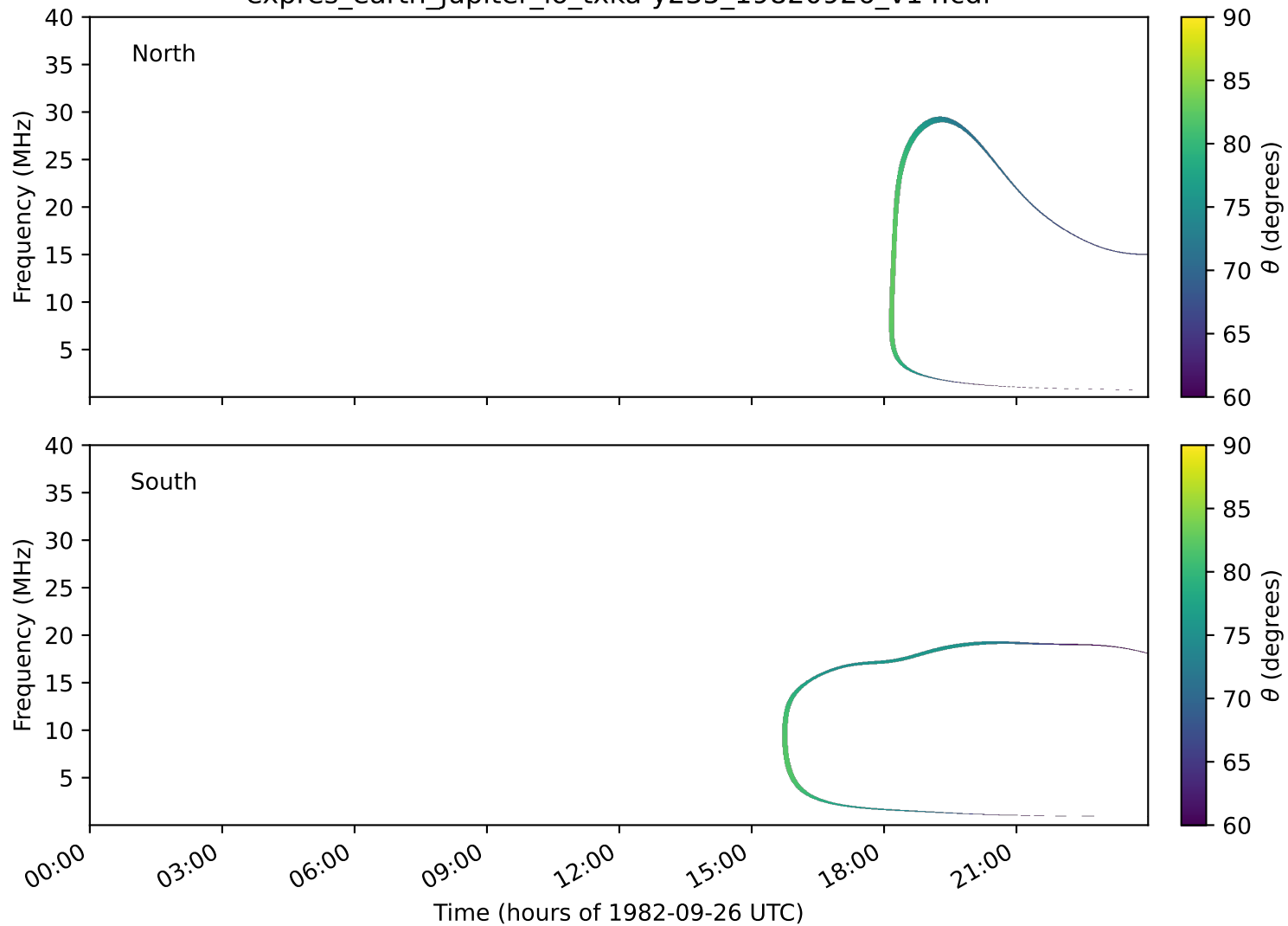
expres_earth_jupiter_io_txka-y235_19820926_v14.cdf
