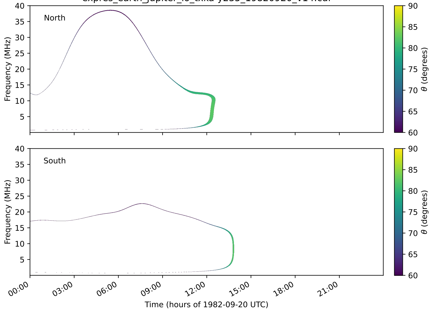
expres_earth_jupiter_io_txka-y235_19820920_v14.cdf
