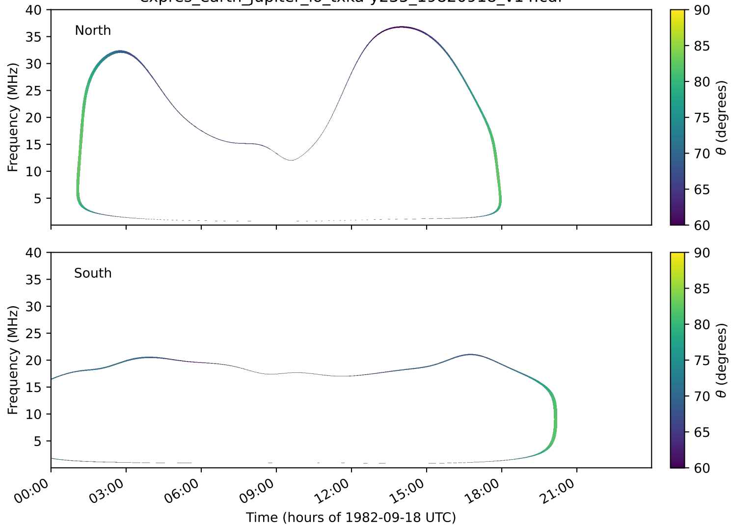
expres_earth_jupiter_io_txka-y235_19820918_v14.cdf
