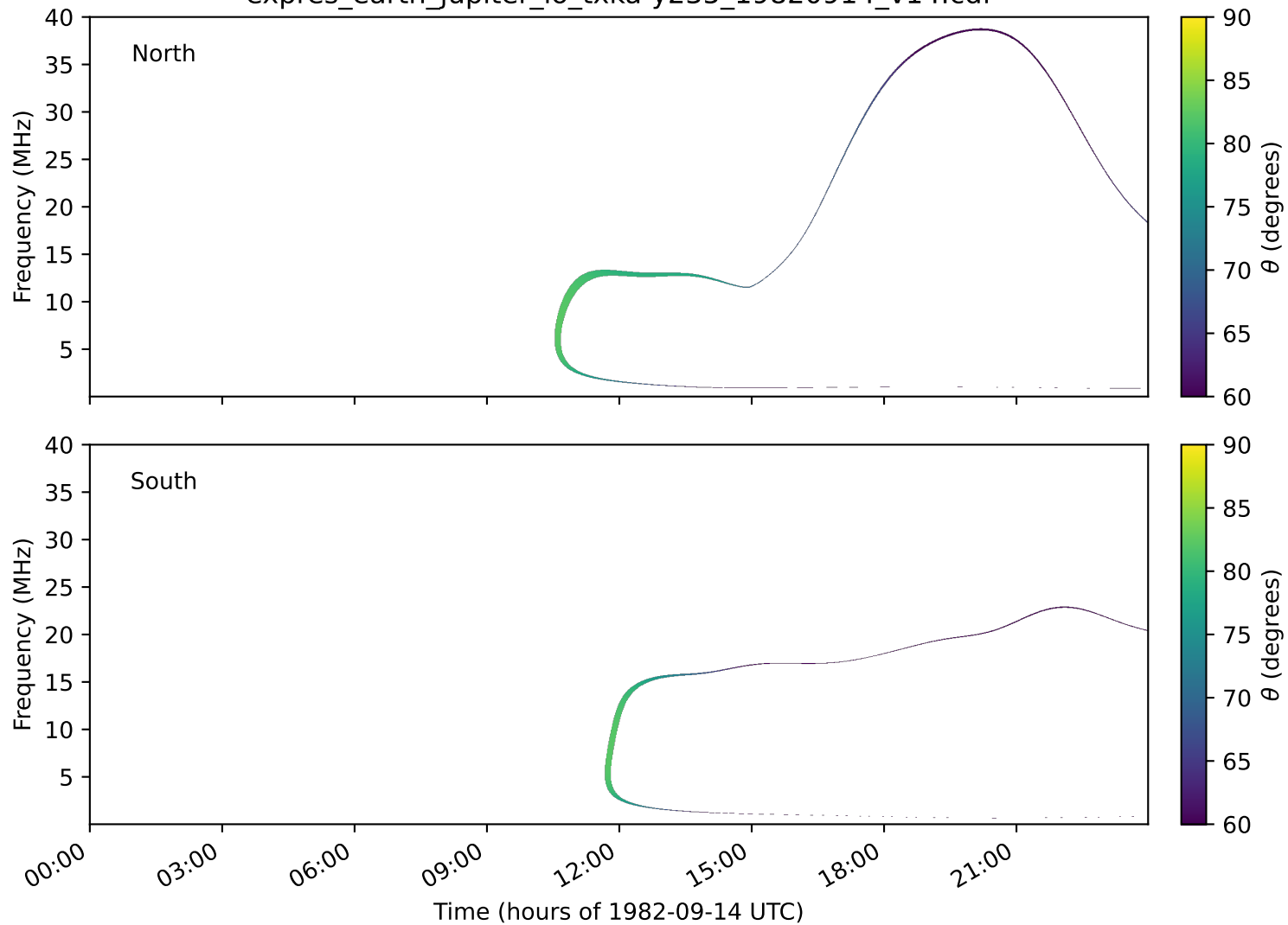
expres_earth_jupiter_io_txka-y235_19820914_v14.cdf
