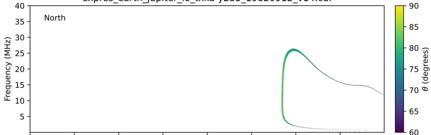
expres_earth_jupiter_io_txka-y235_19820912_v14.cdf
