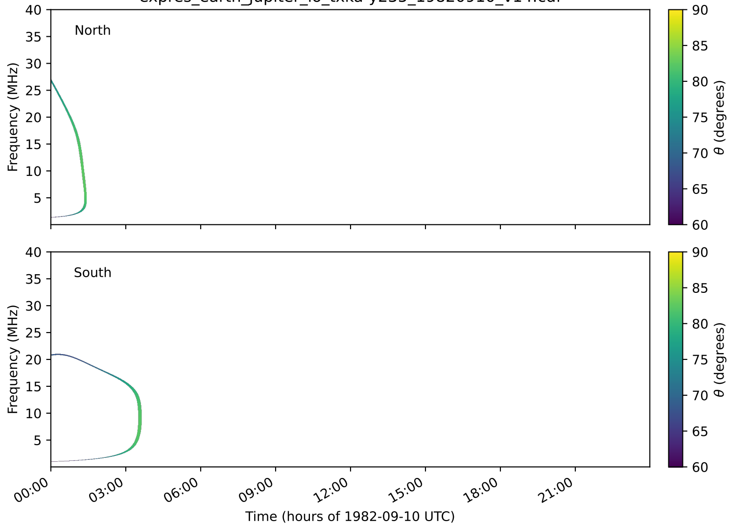
expres_earth_jupiter_io_txka-y235_19820910_v14.cdf
