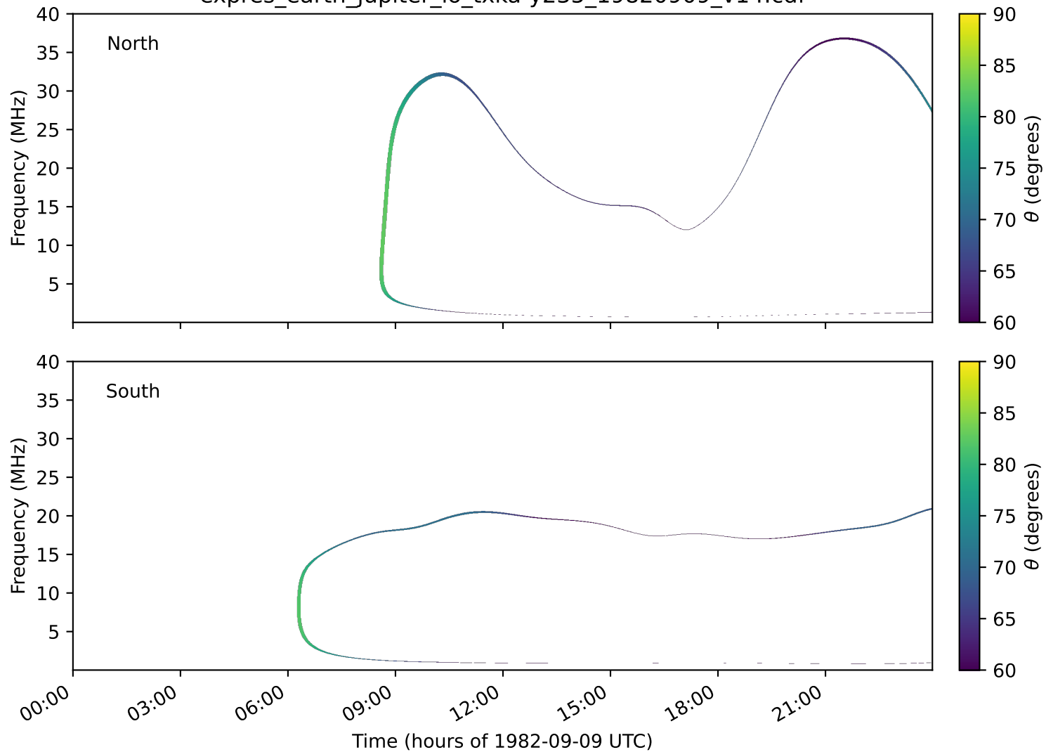
expres_earth_jupiter_io_txka-y235_19820909_v14.cdf
