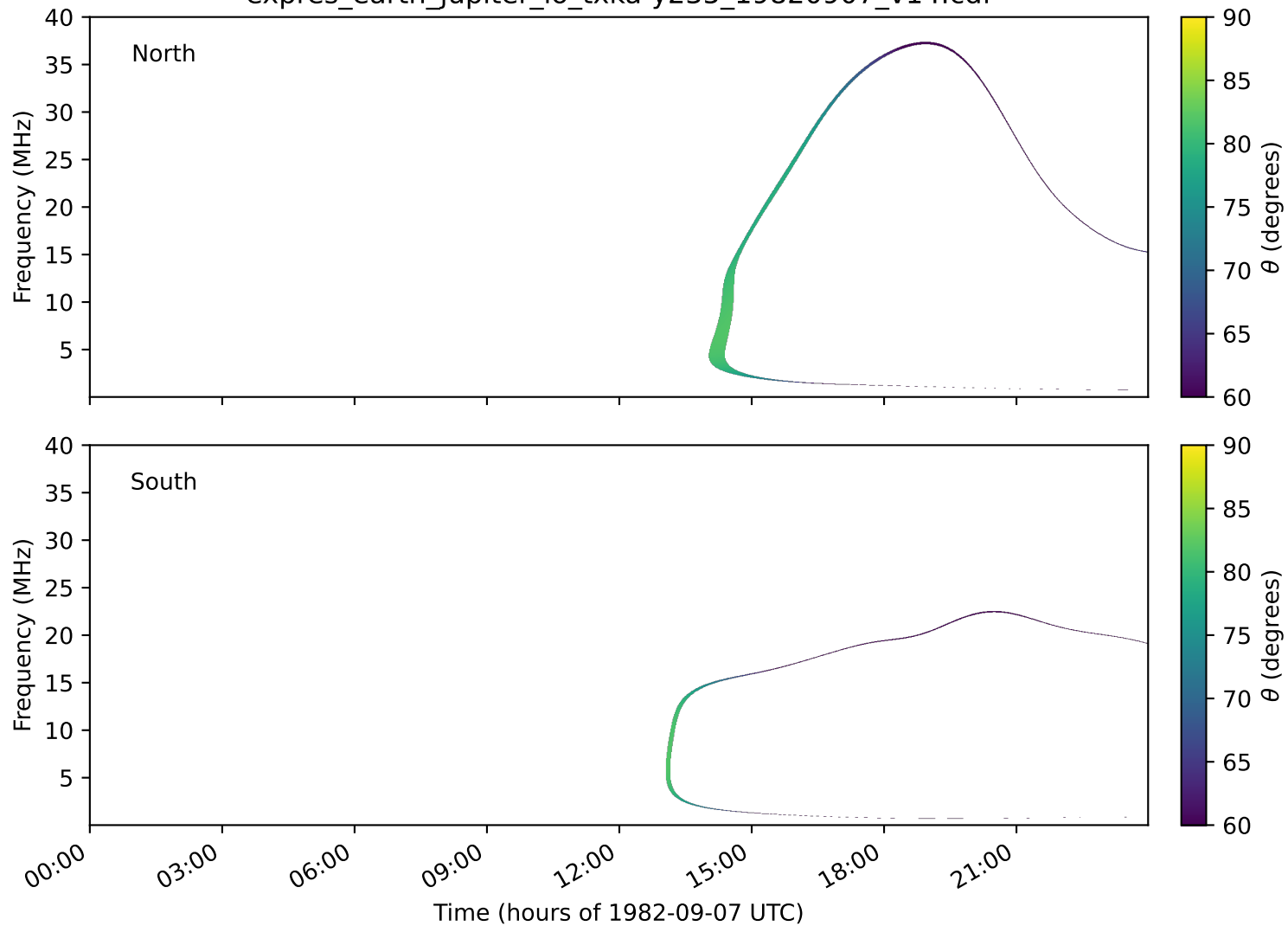
expres_earth_jupiter_io_txka-y235_19820907_v14.cdf
