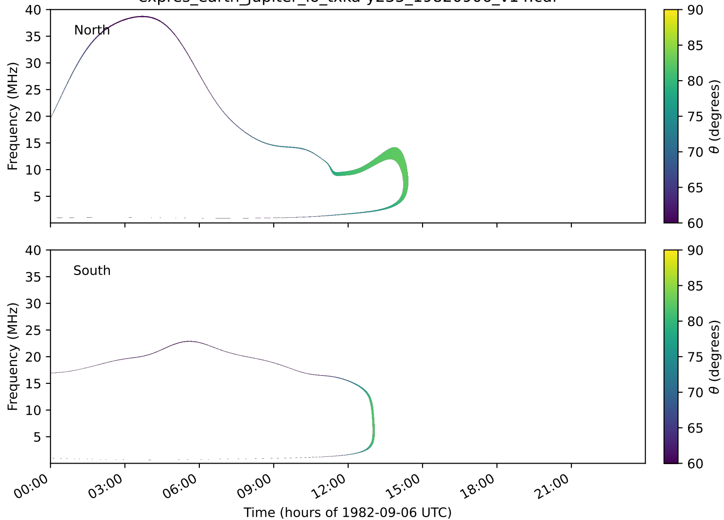
expres_earth_jupiter_io_txka-y235_19820906_v14.cdf
