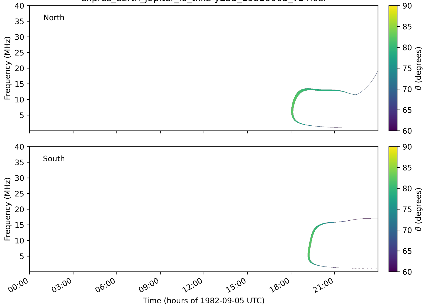
expres_earth_jupiter_io_txka-y235_19820905_v14.cdf
