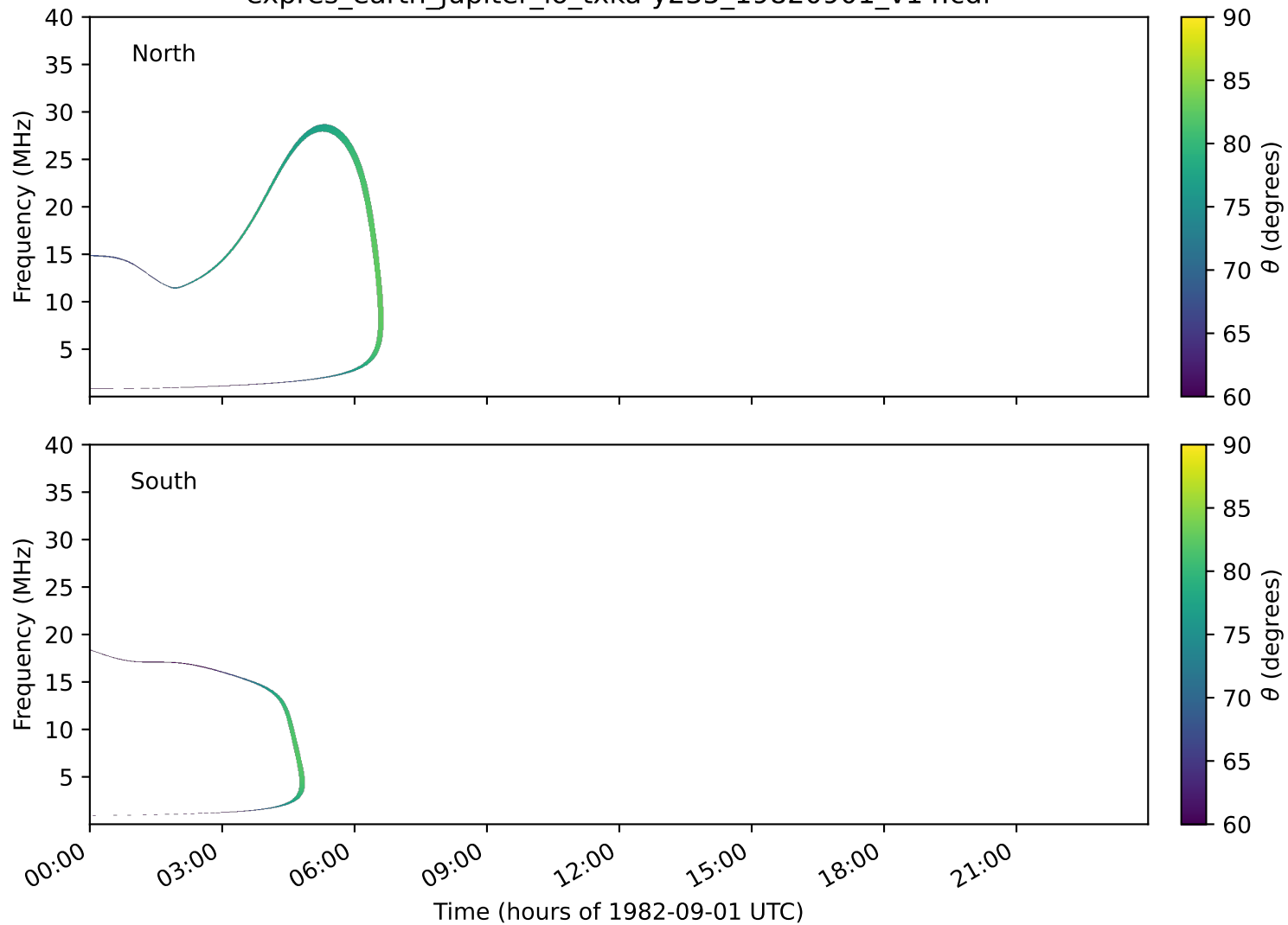
expres_earth_jupiter_io_txka-y235_19820901_v14.cdf
