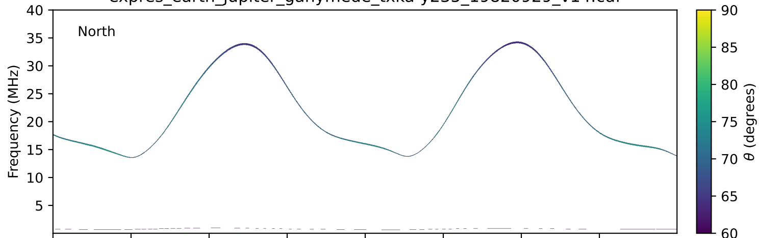
expres_earth_jupiter_ganymede_txka-y235_19820929_v14.cdf
