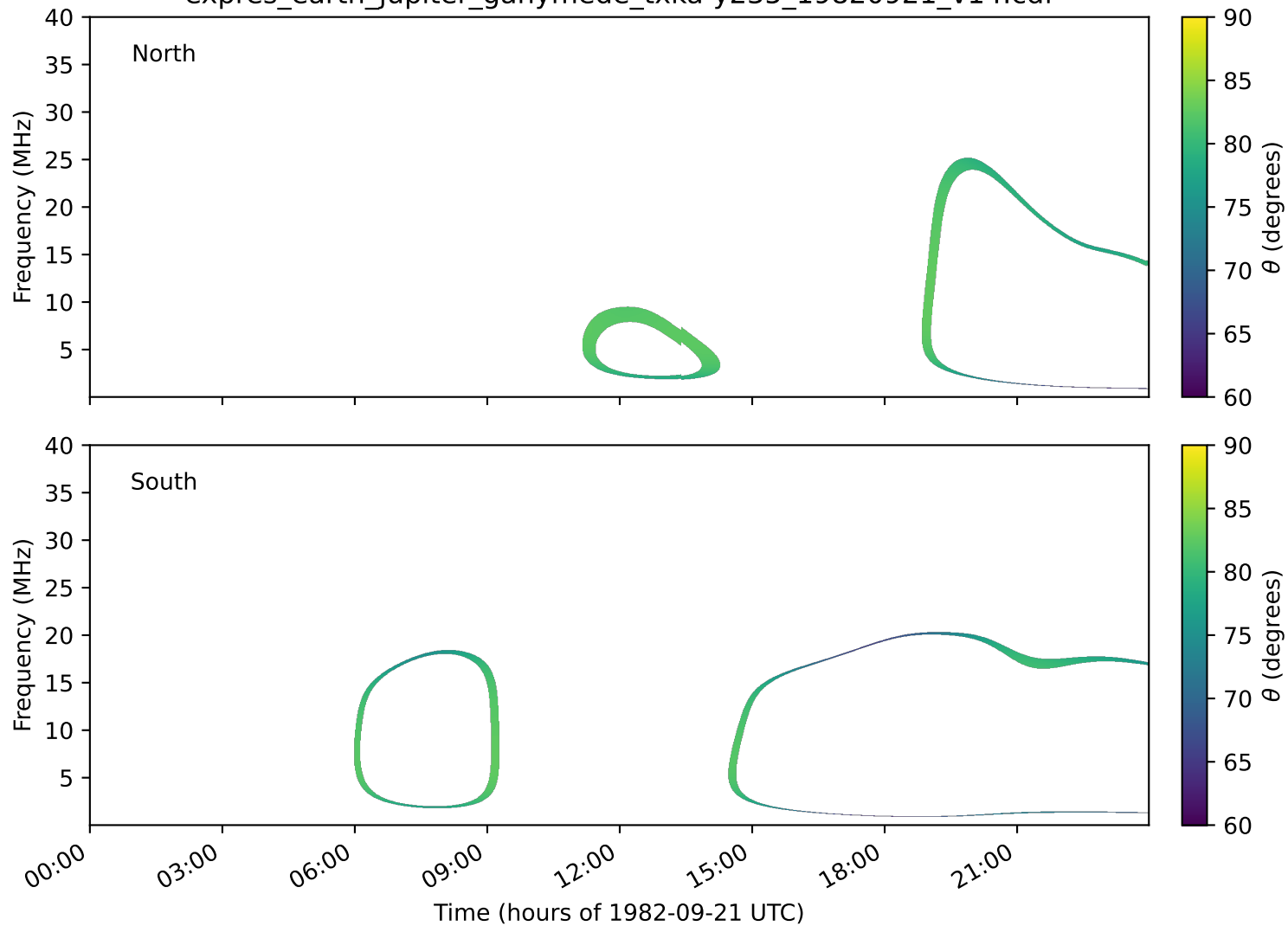
expres_earth_jupiter_ganymede_txka-y235_19820921_v14.cdf
