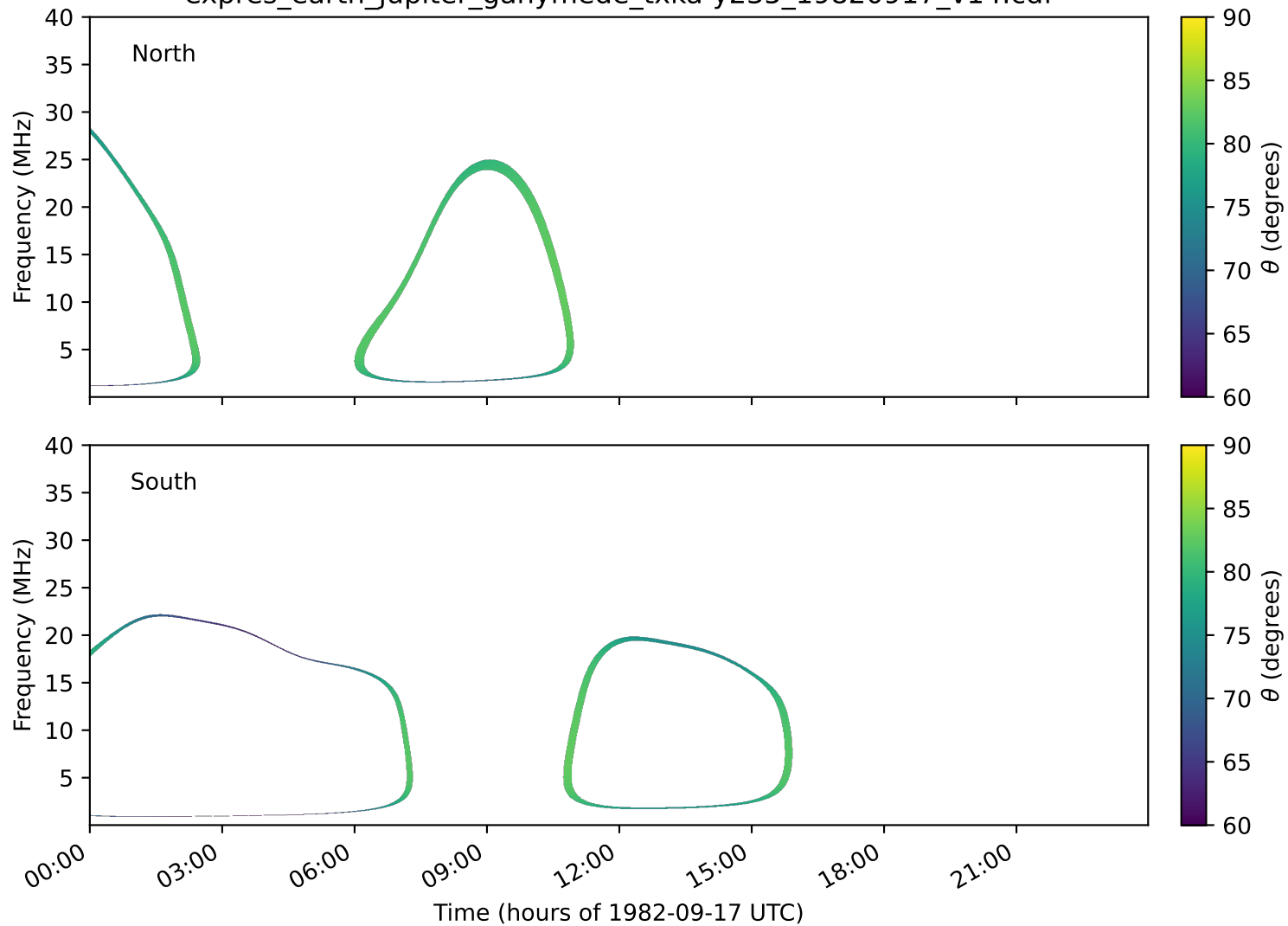
expres_earth_jupiter_ganymede_txka-y235_19820917_v14.cdf
