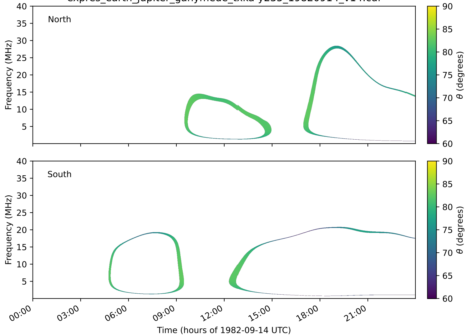
expres_earth_jupiter_ganymede_txka-y235_19820914_v14.cdf
