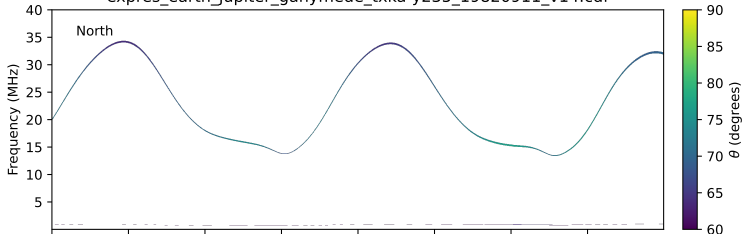
expres_earth_jupiter_ganymede_txka-y235_19820911_v14.cdf
