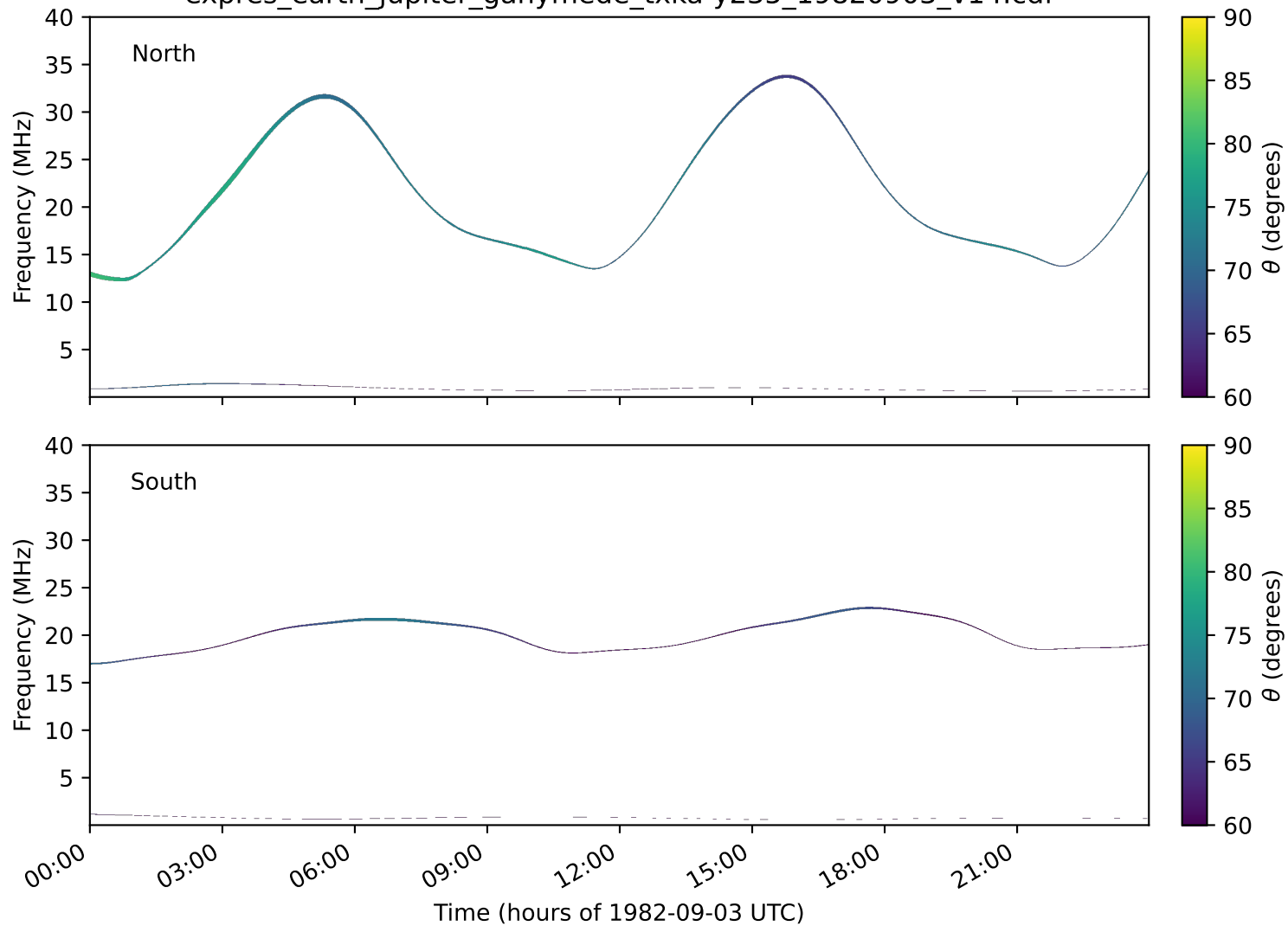
expres_earth_jupiter_ganymede_txka-y235_19820903_v14.cdf
