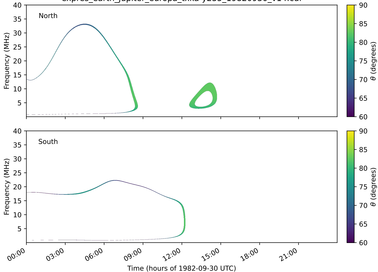
expres_earth_jupiter_europa_txka-y235_19820930_v14.cdf
