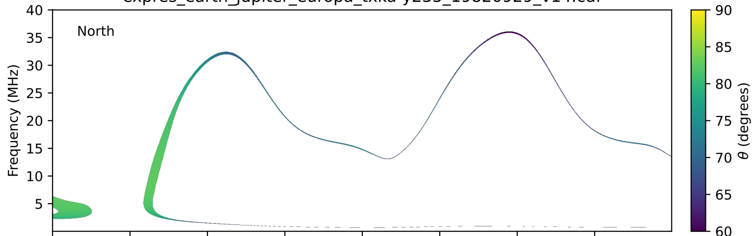
expres_earth_jupiter_europa_txka-y235_19820929_v14.cdf
