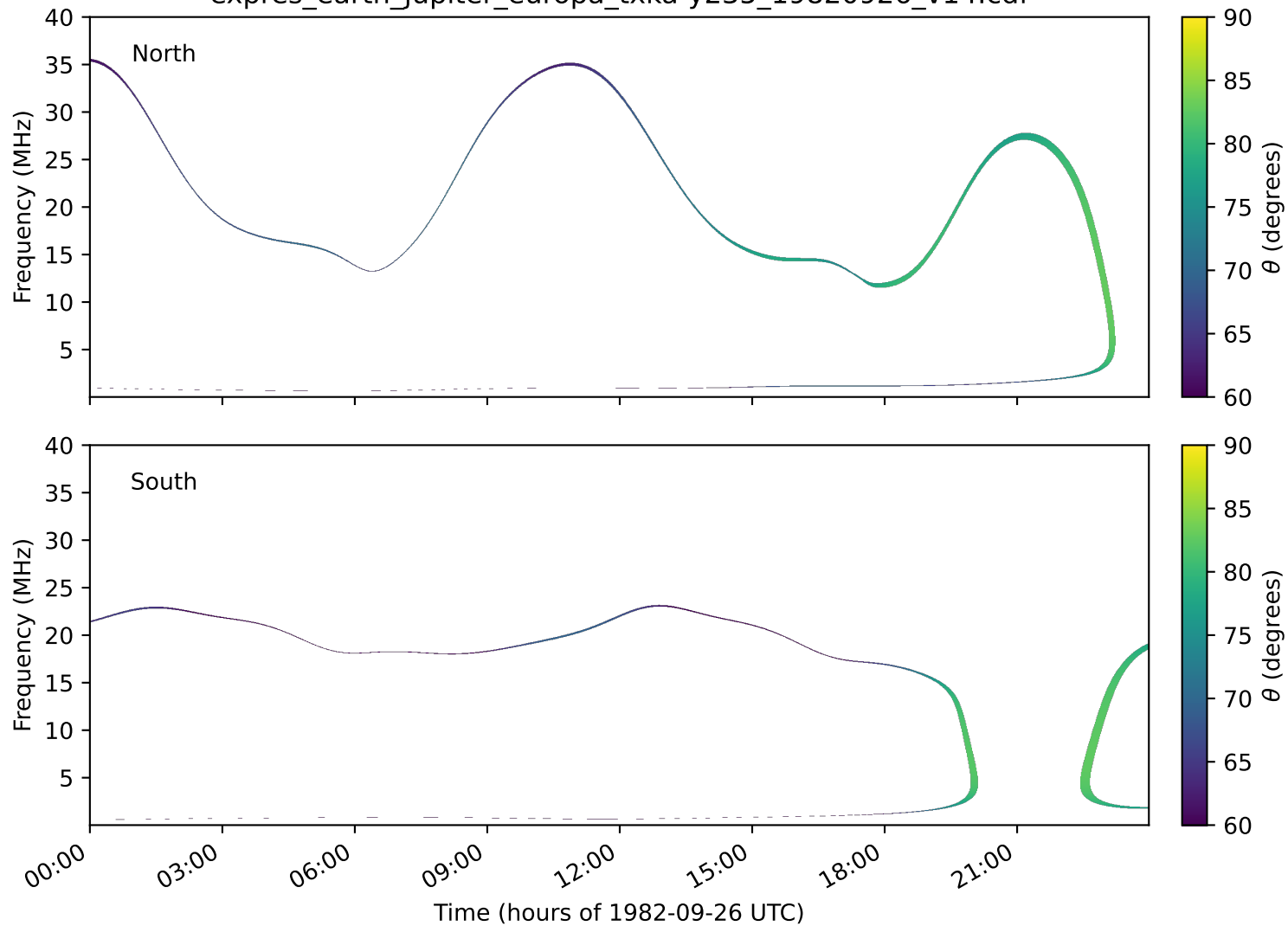
expres_earth_jupiter_europa_txka-y235_19820926_v14.cdf
