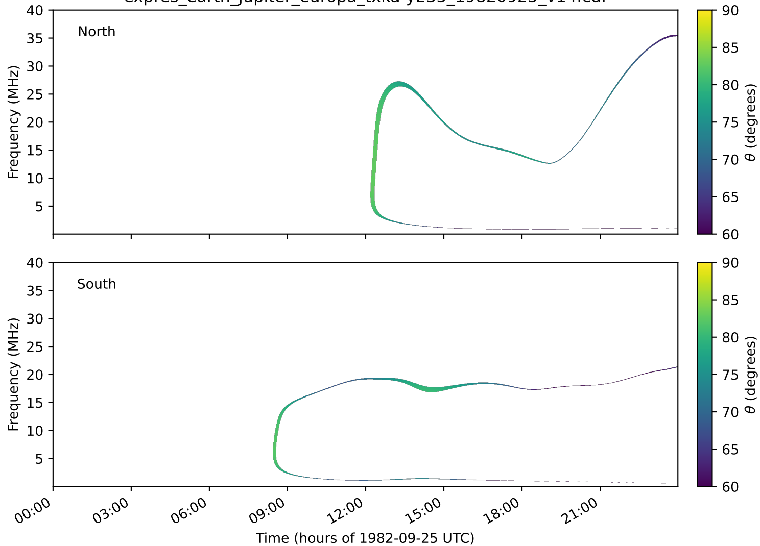
expres_earth_jupiter_europa_txka-y235_19820925_v14.cdf
