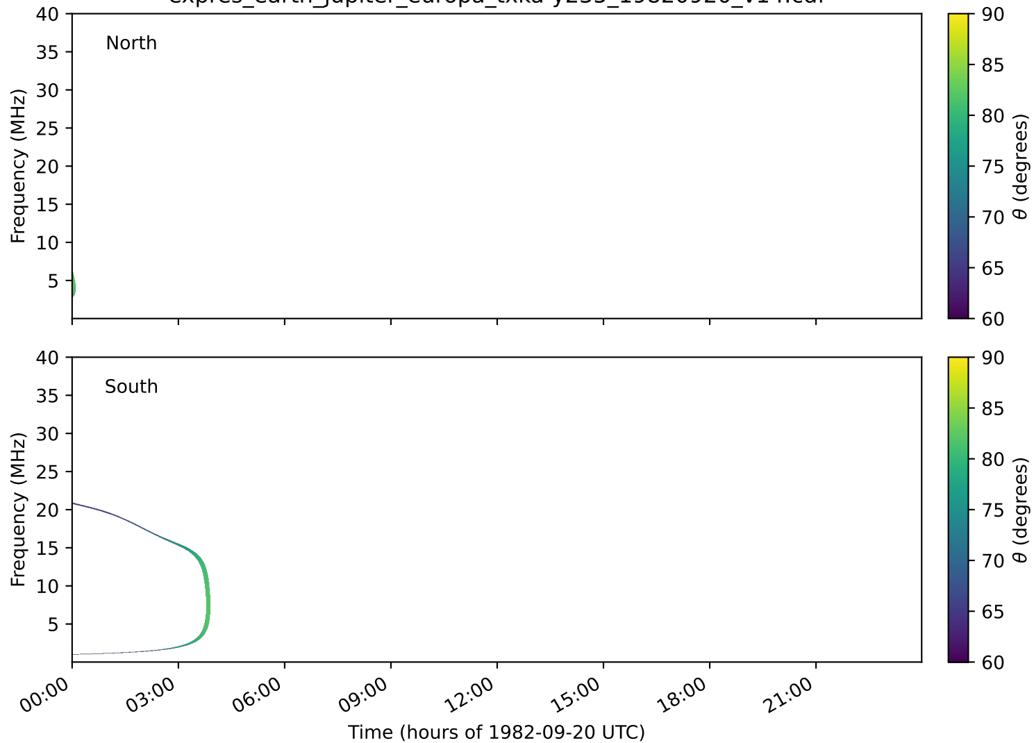
expres_earth_jupiter_europa_txka-y235_19820920_v14.cdf
