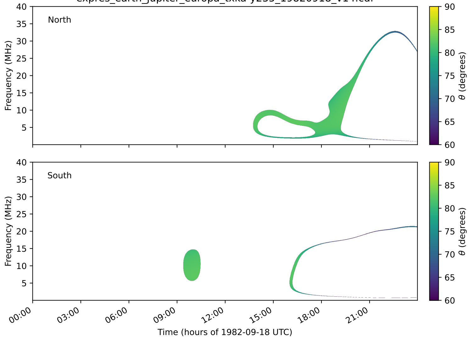
expres_earth_jupiter_europa_txka-y235_19820918_v14.cdf
