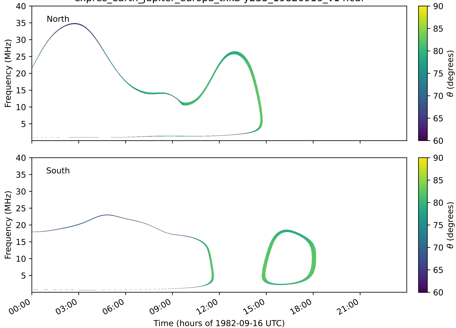
expres_earth_jupiter_europa_txka-y235_19820916_v14.cdf
