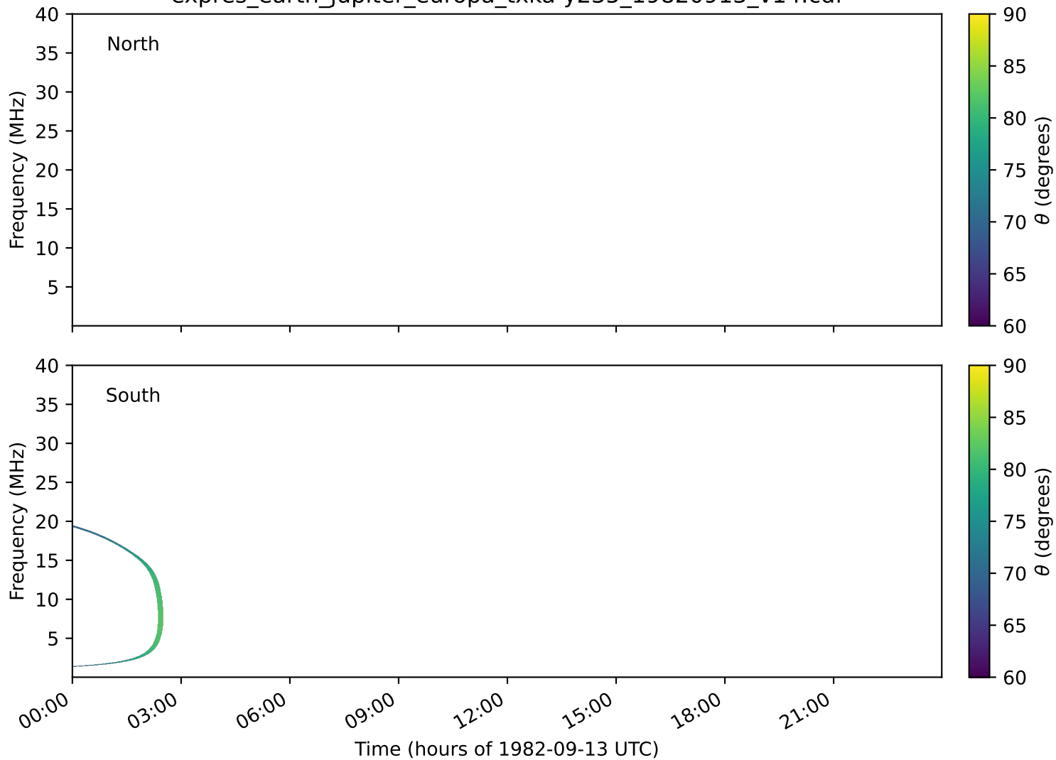
expres_earth_jupiter_europa_txka-y235_19820913_v14.cdf
