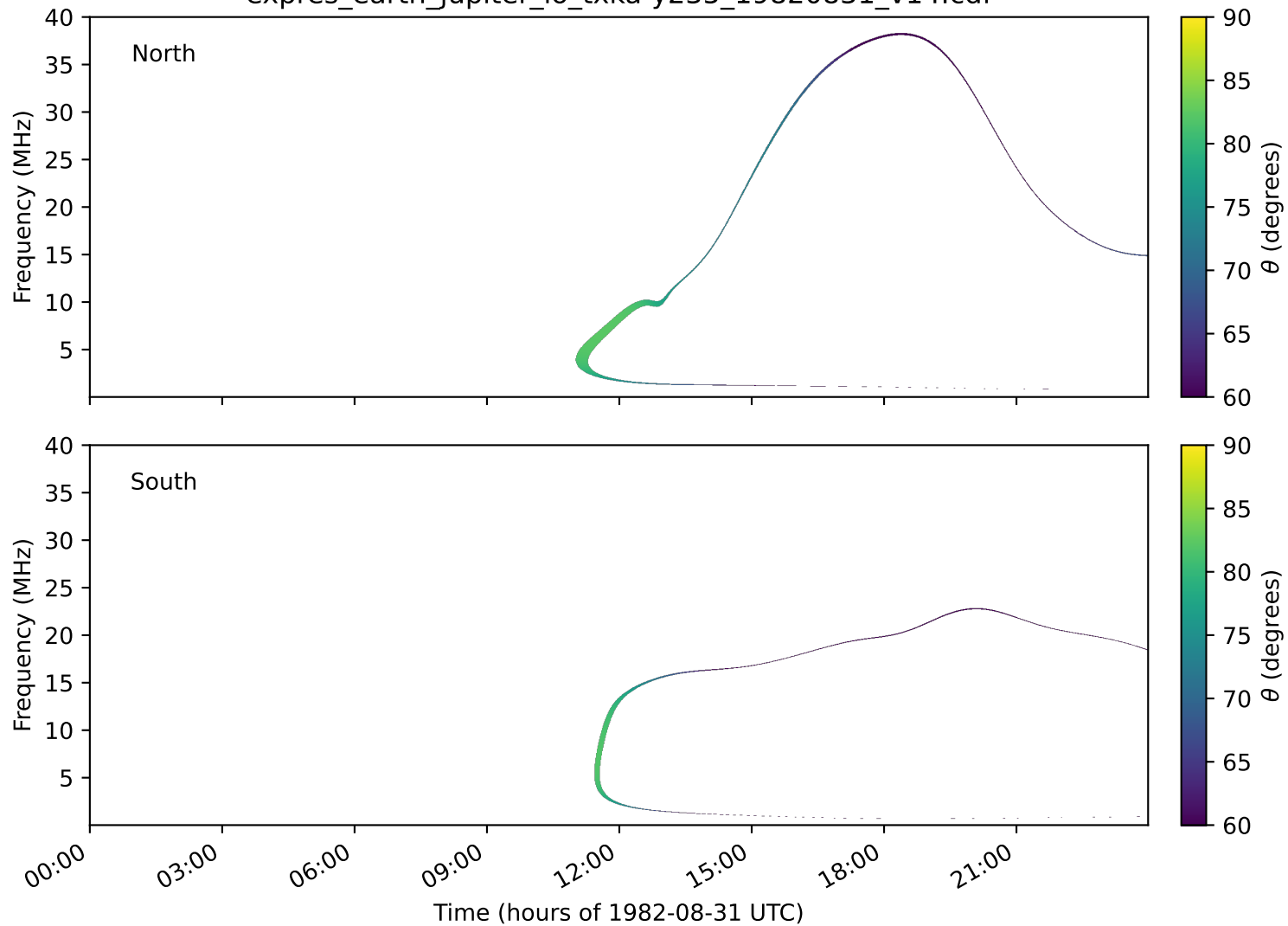
expres_earth_jupiter_io_txka-y235_19820831_v14.cdf
