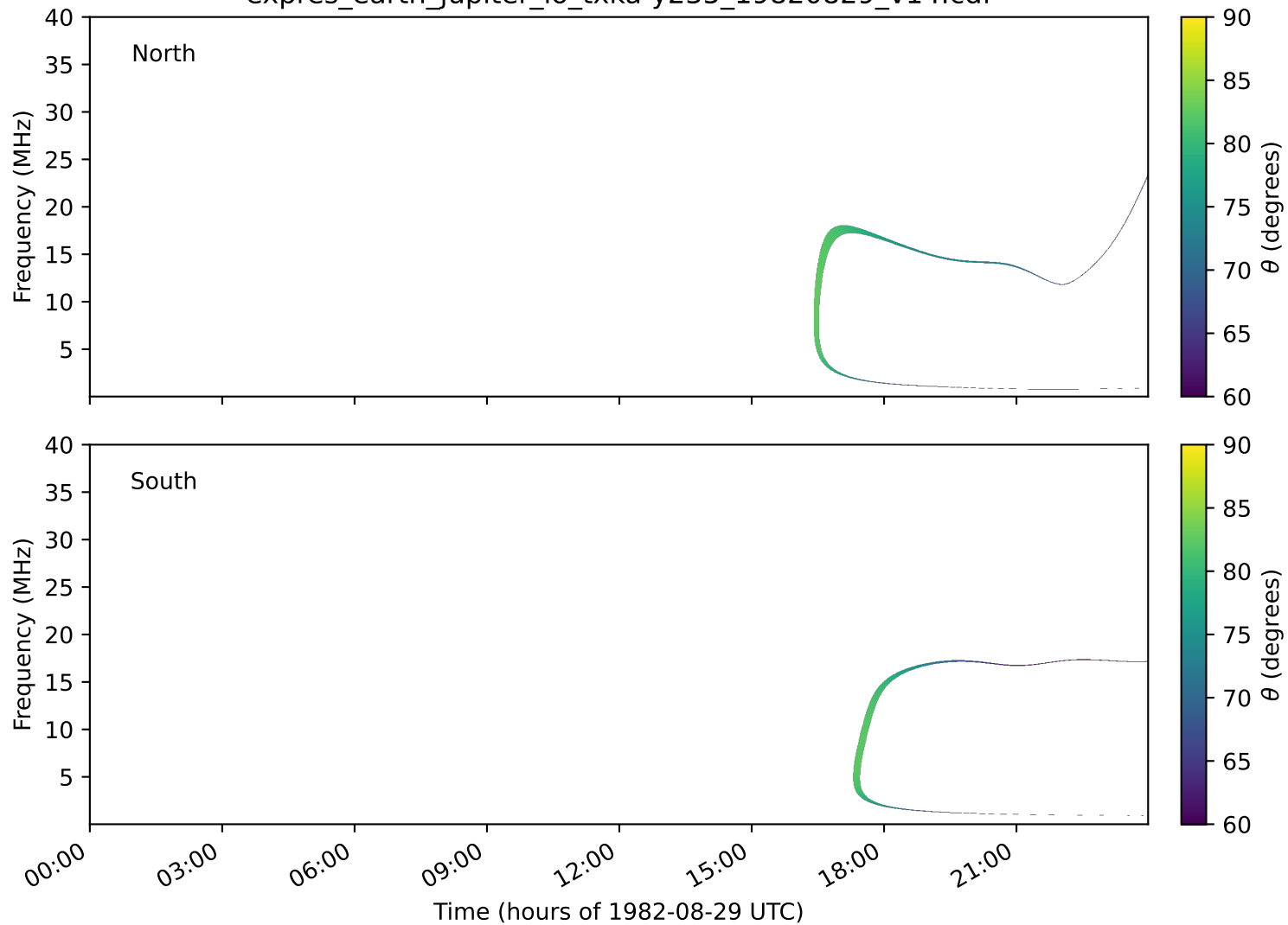
expres_earth_jupiter_io_txka-y235_19820829_v14.cdf
