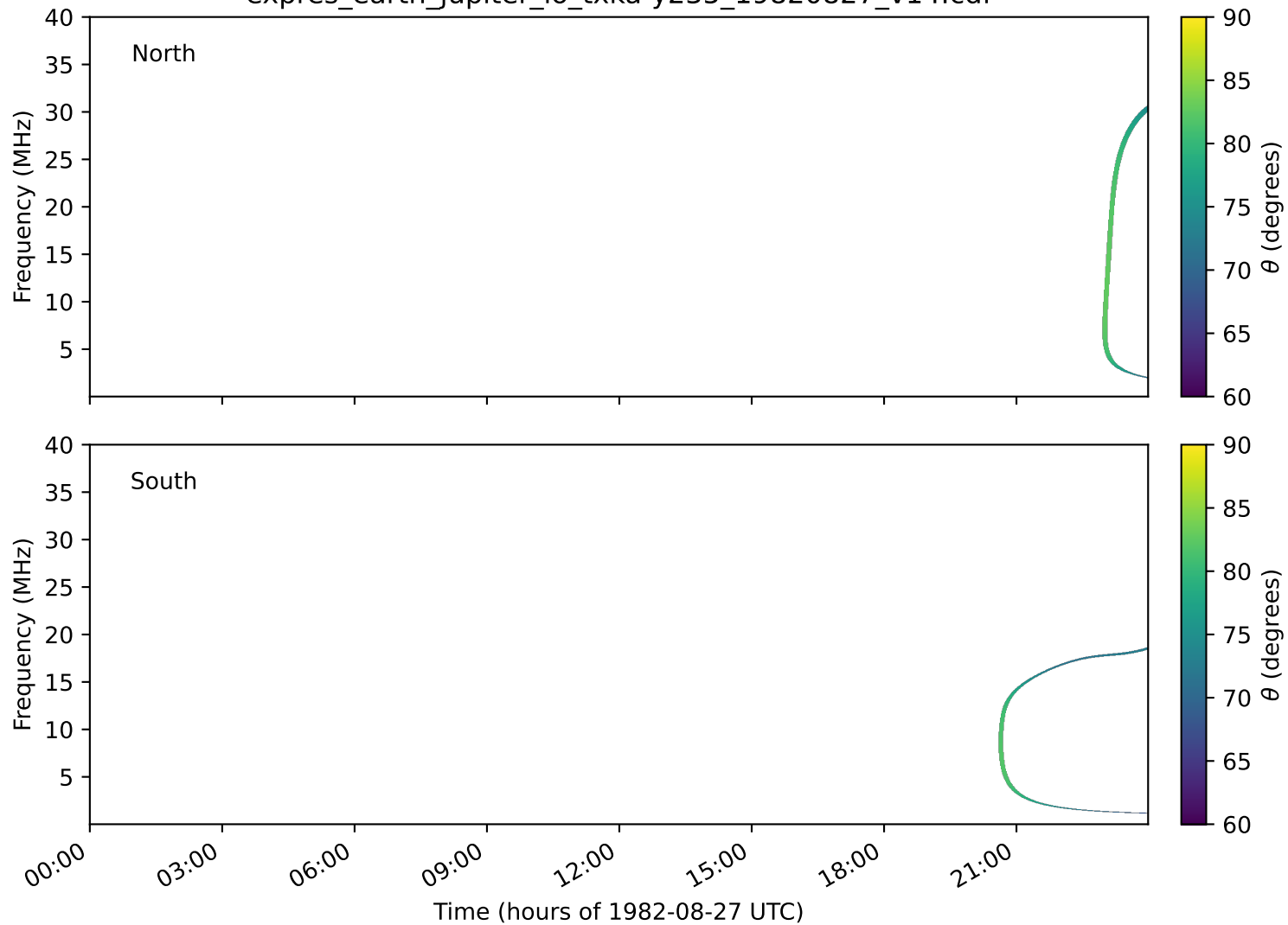
expres_earth_jupiter_io_txka-y235_19820827_v14.cdf
