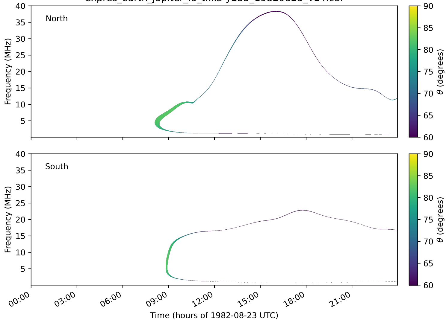
expres_earth_jupiter_io_txka-y235_19820823_v14.cdf
