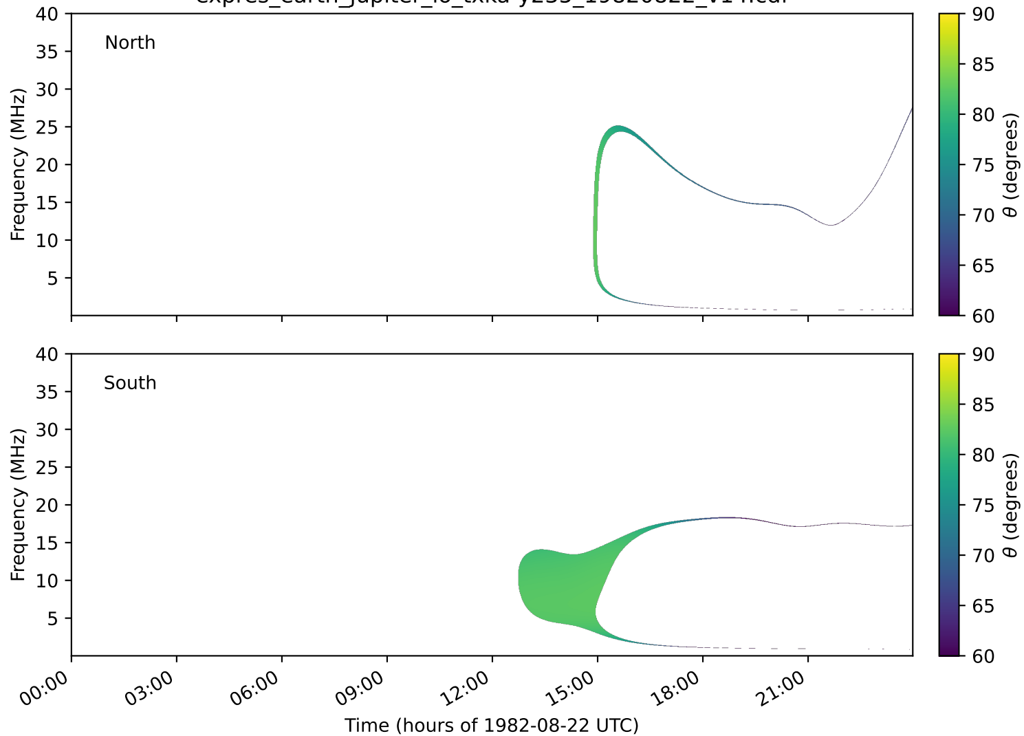
expres_earth_jupiter_io_txka-y235_19820822_v14.cdf
