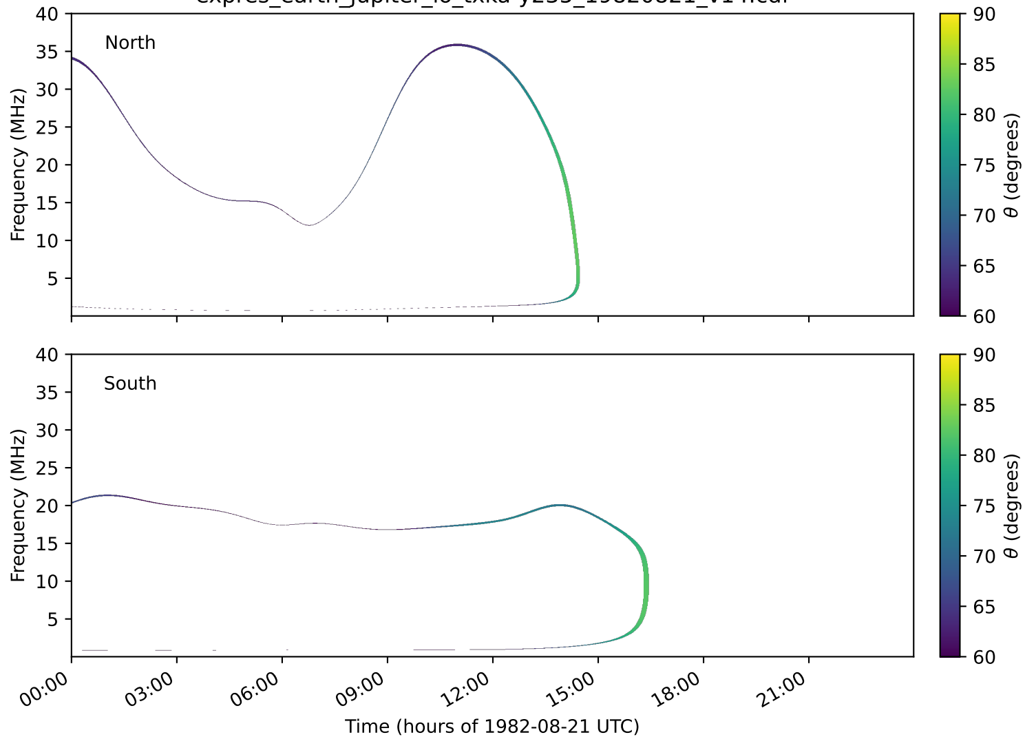
expres_earth_jupiter_io_txka-y235_19820821_v14.cdf
