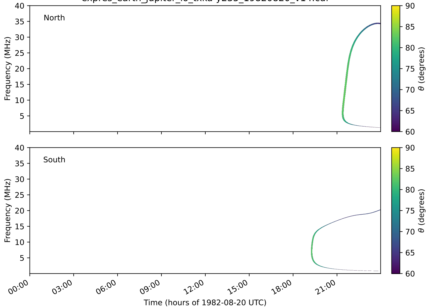
expres_earth_jupiter_io_txka-y235_19820820_v14.cdf
