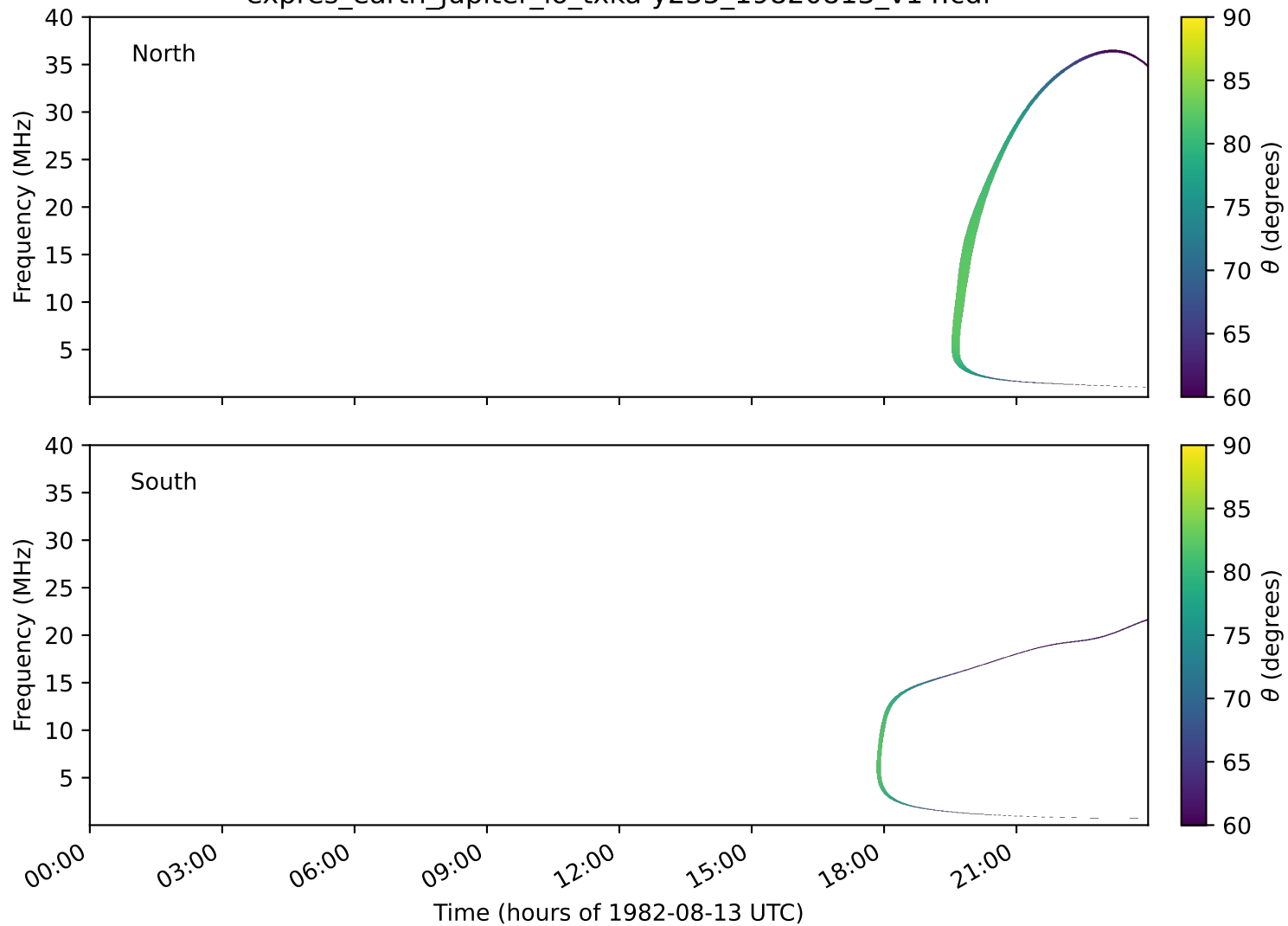
expres_earth_jupiter_io_txka-y235_19820813_v14.cdf
