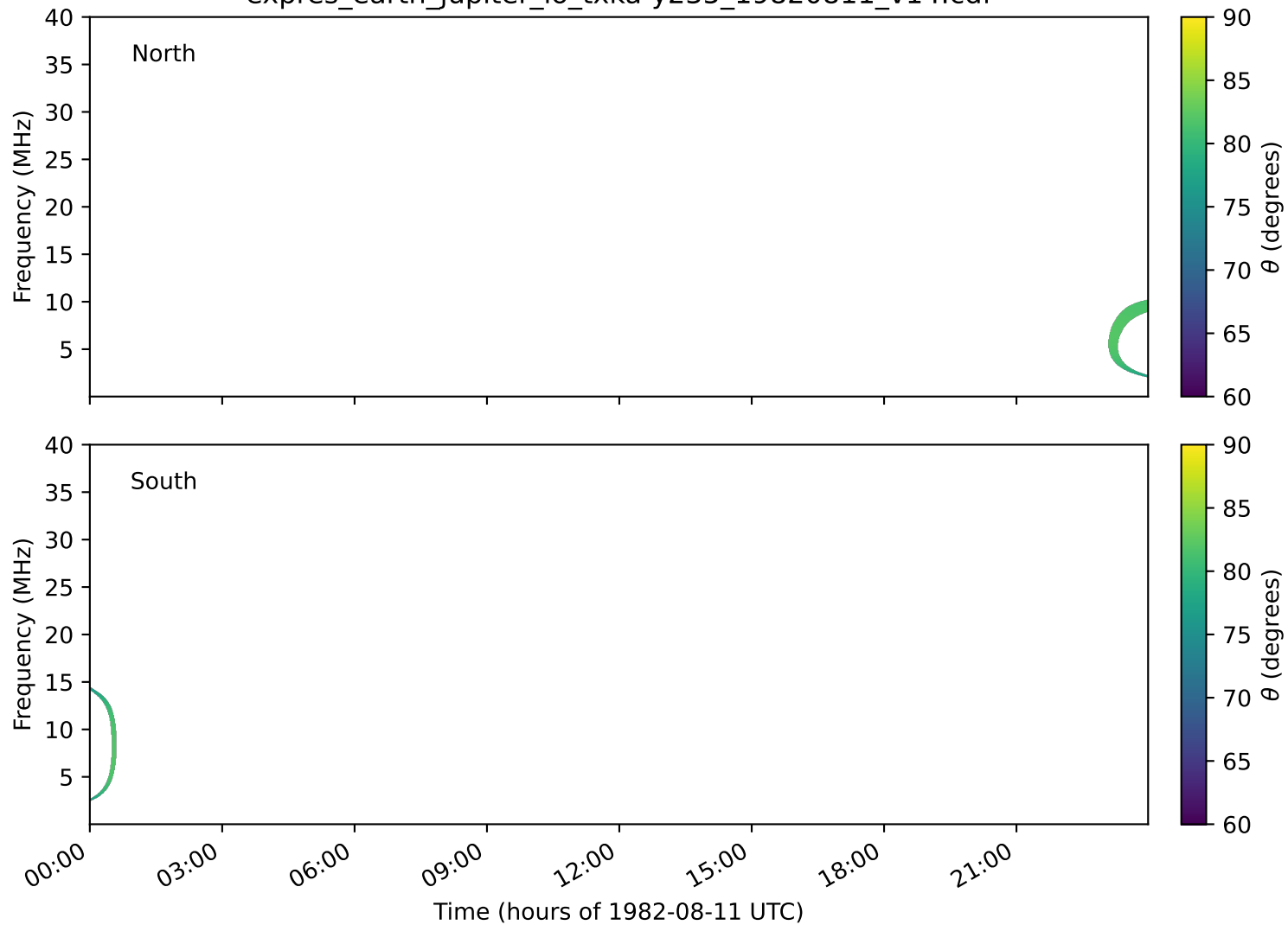
expres_earth_jupiter_io_txka-y235_19820811_v14.cdf
