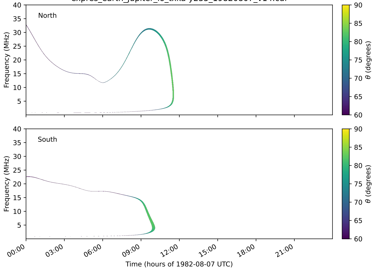
expres_earth_jupiter_io_txka-y235_19820807_v14.cdf
