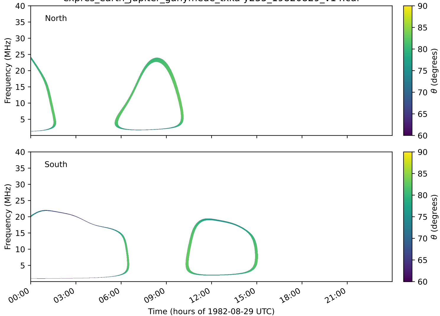
expres_earth_jupiter_ganymede_txka-y235_19820829_v14.cdf
