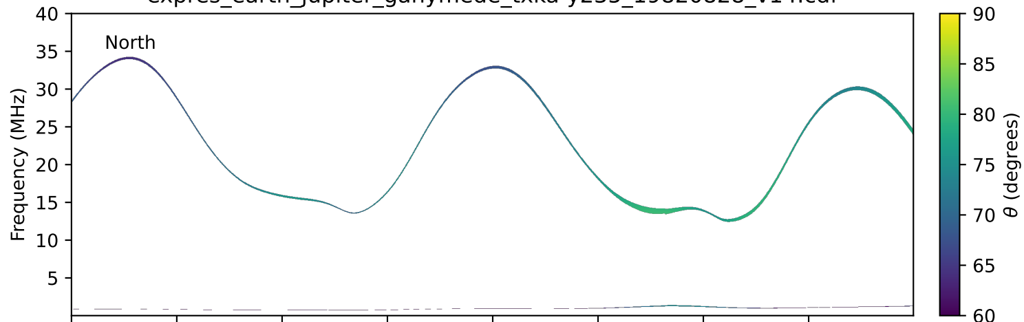
expres_earth_jupiter_ganymede_txka-y235_19820828_v14.cdf
