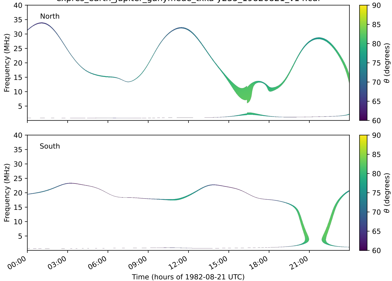
expres_earth_jupiter_ganymede_txka-y235_19820821_v14.cdf
