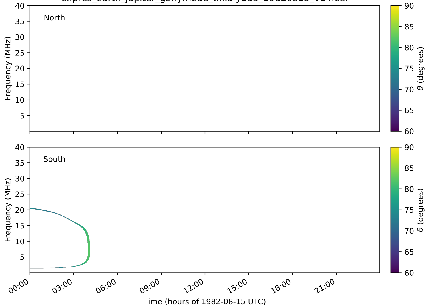
expres_earth_jupiter_ganymede_txka-y235_19820815_v14.cdf
