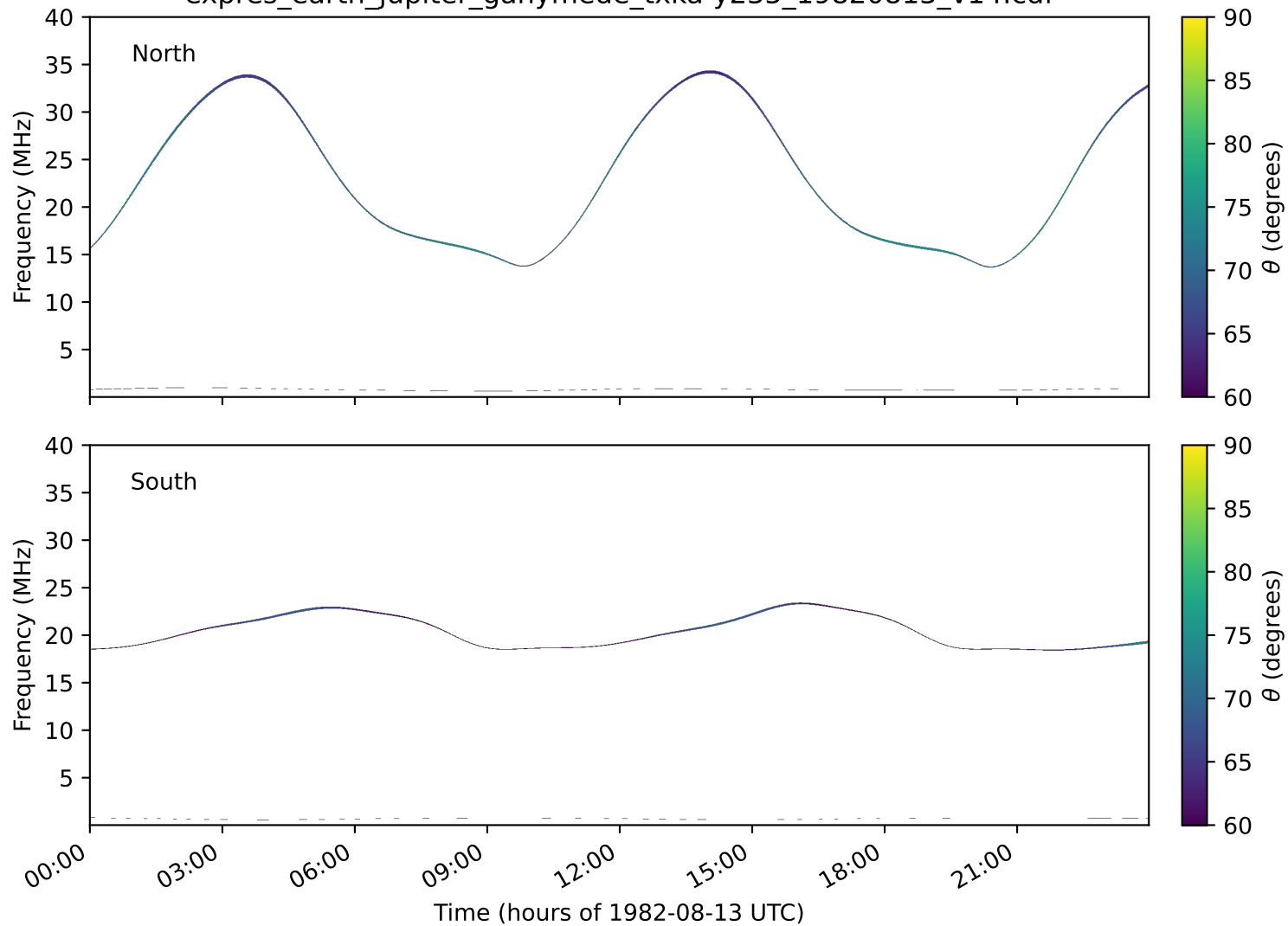
expres_earth_jupiter_ganymede_txka-y235_19820813_v14.cdf
