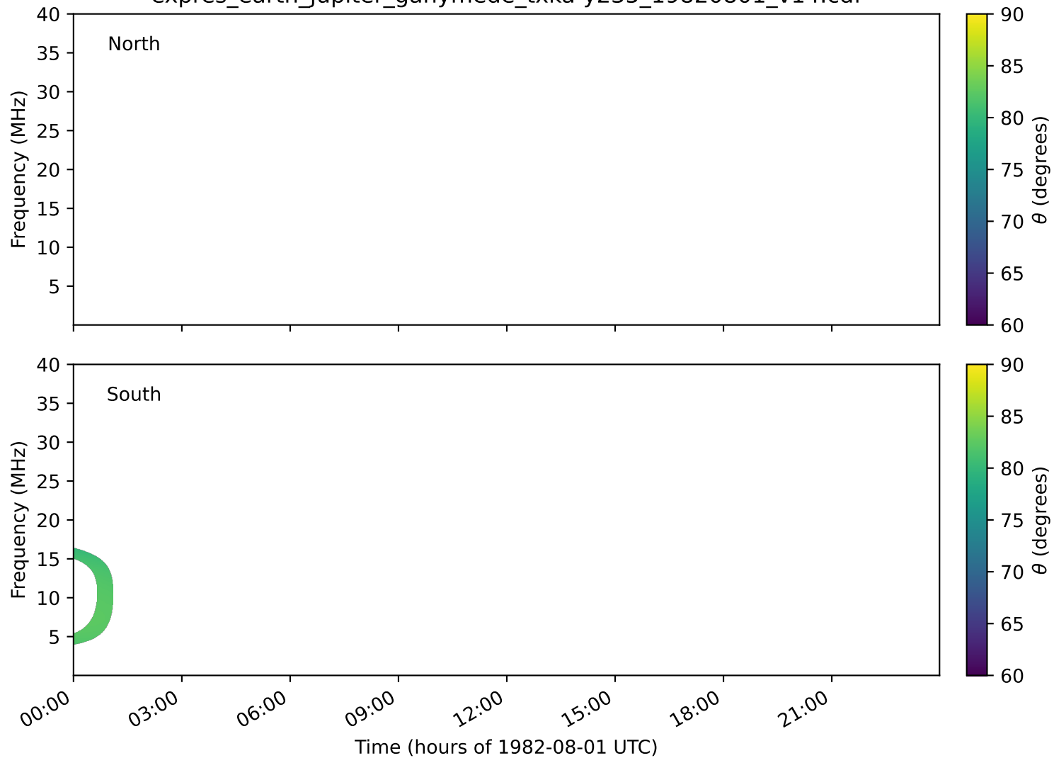
expres_earth_jupiter_ganymede_txka-y235_19820801_v14.cdf
