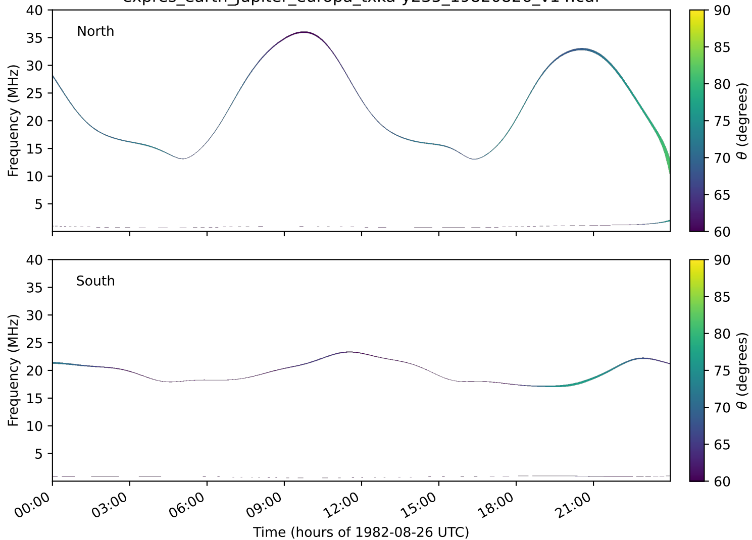
expres_earth_jupiter_europa_txka-y235_19820826_v14.cdf
