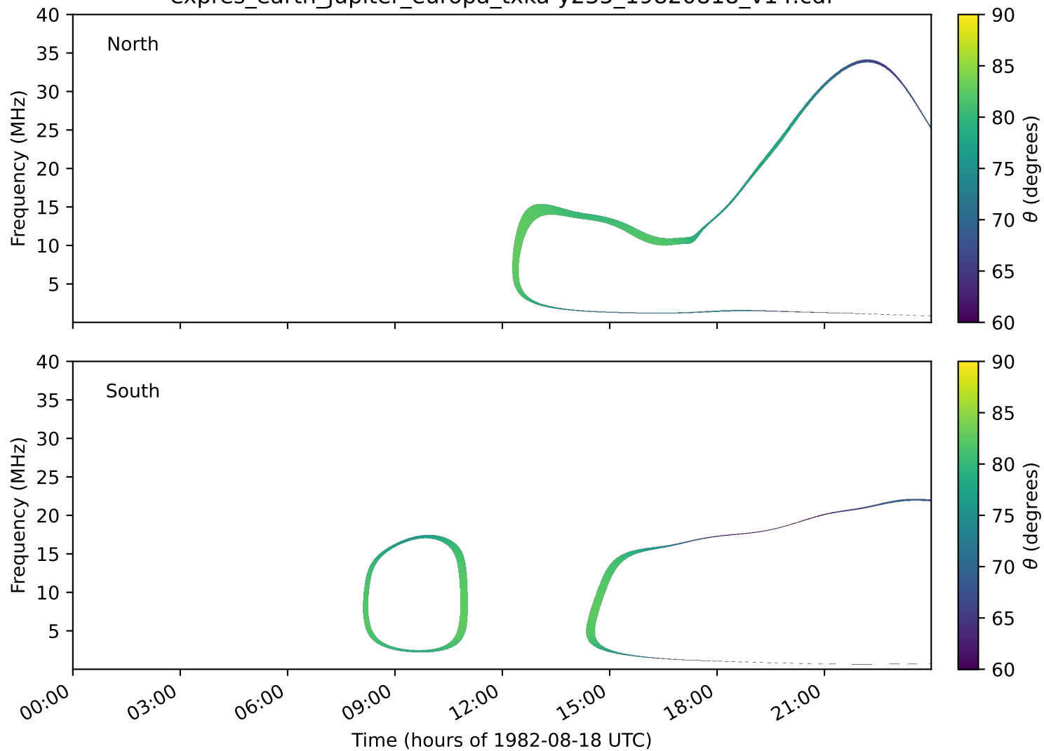
expres_earth_jupiter_europa_txka-y235_19820818_v14.cdf
